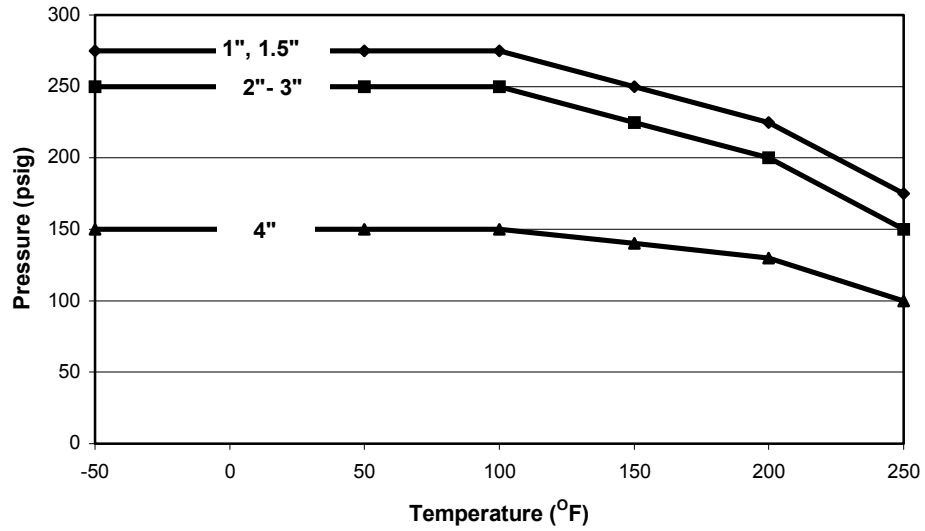
Pressure/Temperature Rating
