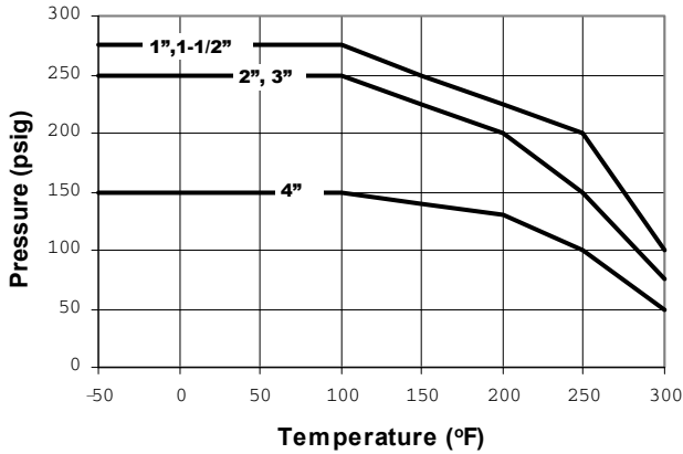
Pressure/Temperature Rating
