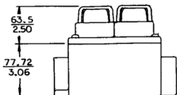
TWO GANG DOUBLE PILOT LIGHT EACH GANG, 4-RED PILOT L16HTS THROUGH FEED
